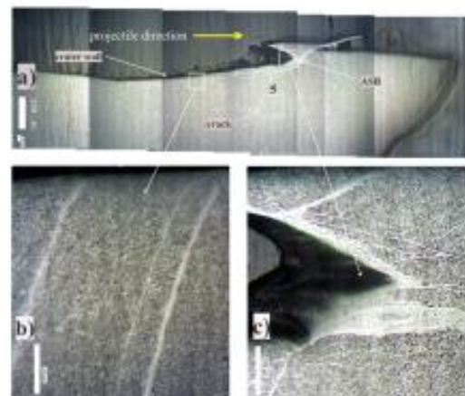
Fig. 8 Microstructure of hard plate.
